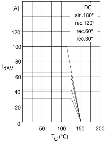
Maximum forward current at case temperature
