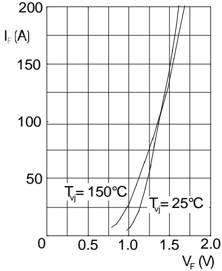
Forward current versus voltage drop per diode
