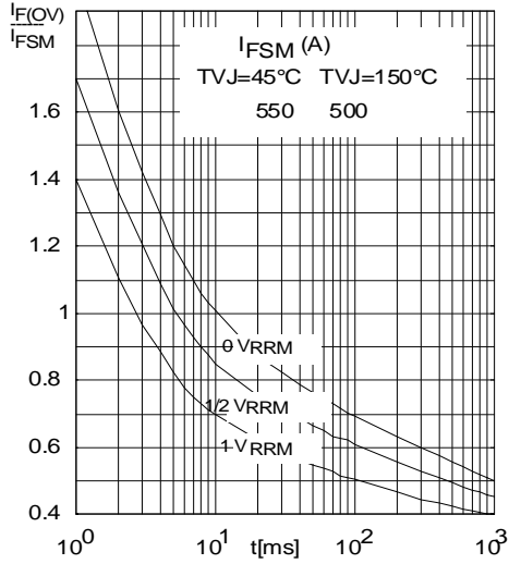
Surge overload current per diode I_{FSM} : Crest value t: duration
