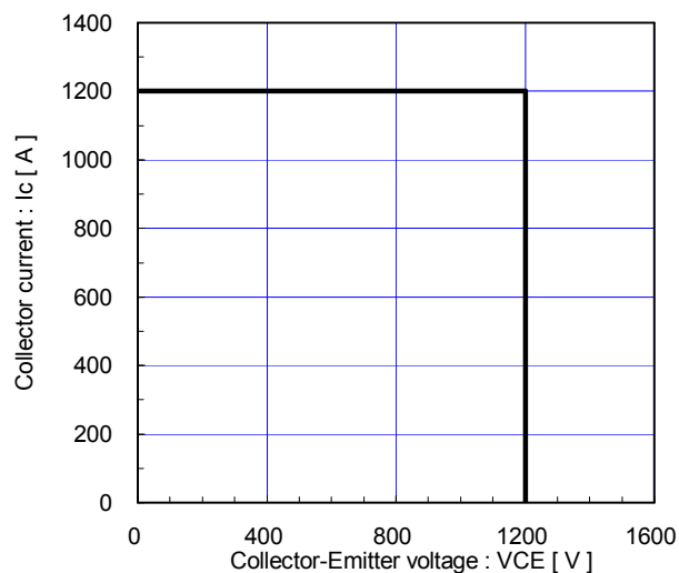
Reverse bias safe operating area (max.) +V_{GE}=15V, -V_{GE} \leq 15V, R_G \geq 0.6\Omega, T_J \leq 125^\circ C
