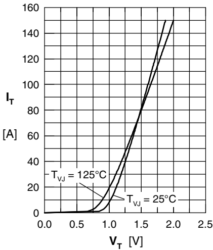
Fig. 1 Forward characteristics
