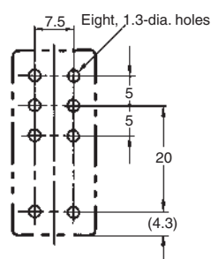
Mounting Holes (Bottom View)
