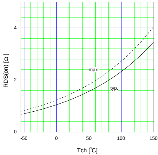
Drain-source on-state resistance R_{DS(on)} = f(T_{ch}) : I_D = 4.5A, V_{GS} = 10V
