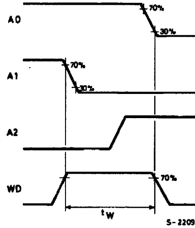
Definition of WRITE DISABLE ON Time
