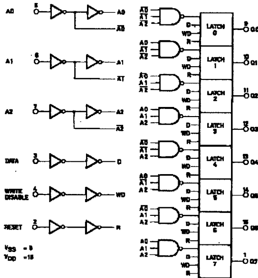
1 of 8 latches
