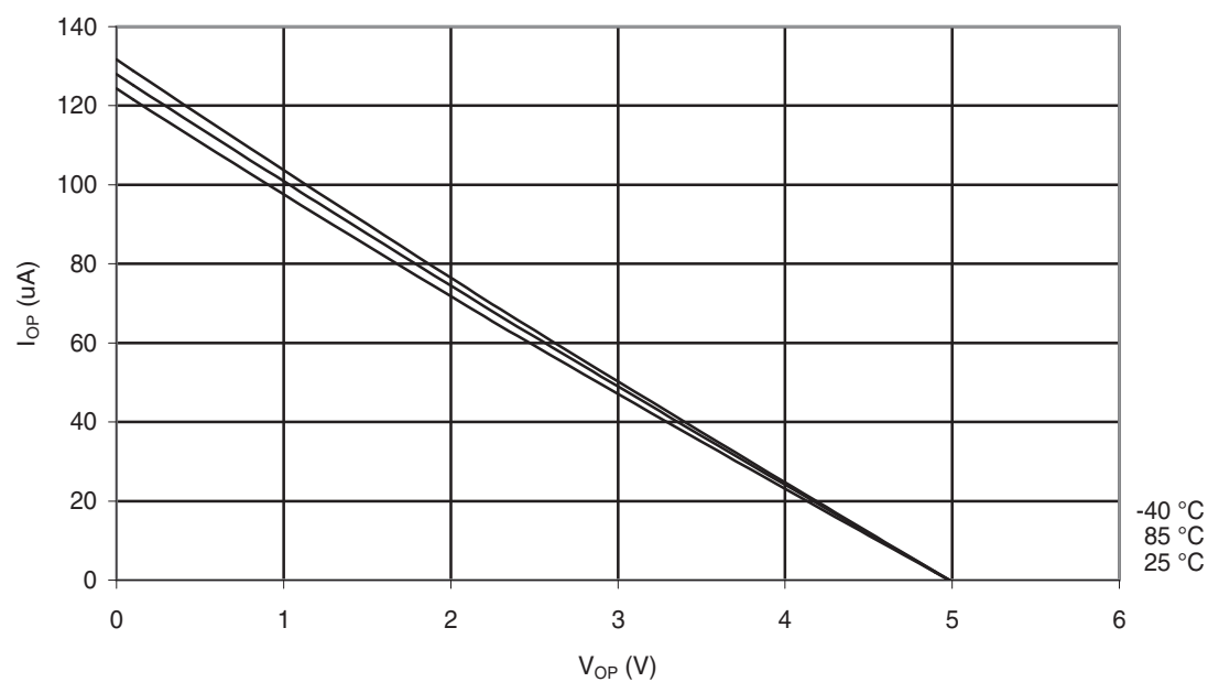
Figure 28-25. I/O Pin Pull-up Resistor Current vs. Input Voltage ( V_{CC} = 5V )
