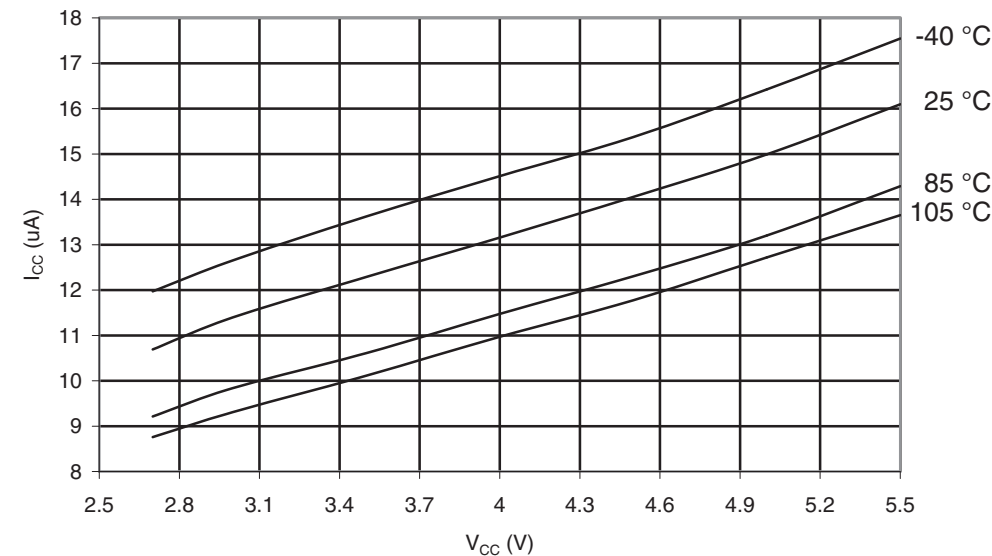
Figure 29-50. Brown-out Detector Current vs. V_{CC}
