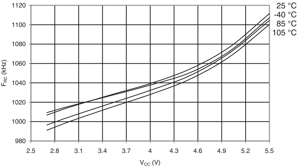
Figure 29-36. Watchdog Oscillator Frequency vs. V_{CC}
