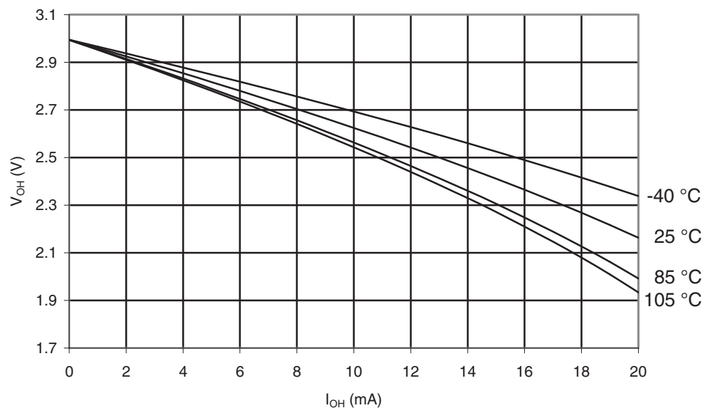
Figure 29-20. I/O Pin Output Voltage vs. Source Current ( V_{CC} = 3V )
