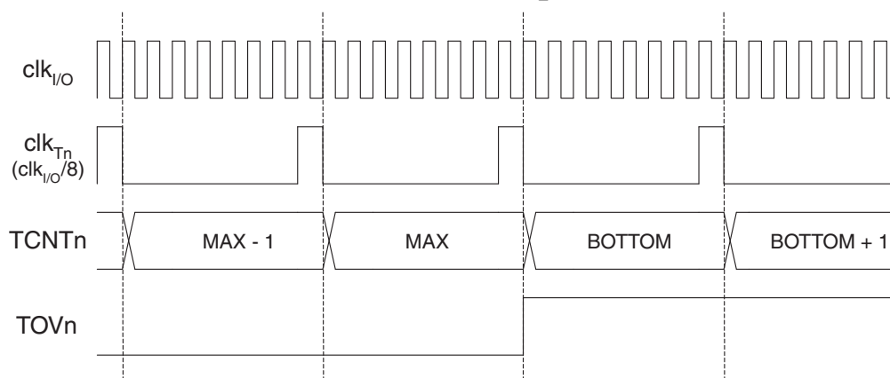
Figure 18-9. Timer/Counter Timing Diagram, with Prescaler ( f_{\text{clk}_{I/O}}/8 )
