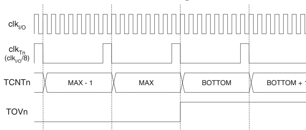
Figure 15-4. Timer/Counter Timing Diagram, with Prescaler ( f_{\text{clk}_{I/O}}/8 )
