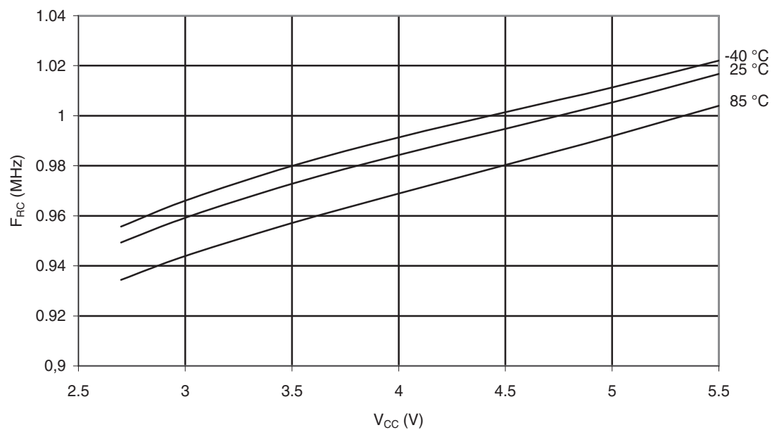
Figure 28-62. Calibrated 1MHz RC Oscillator Frequency vs. V_{CC}
