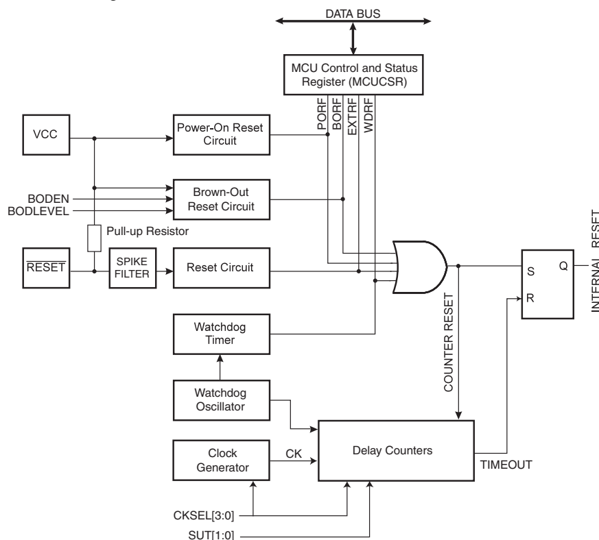
Figure 10-1. Reset Logic
