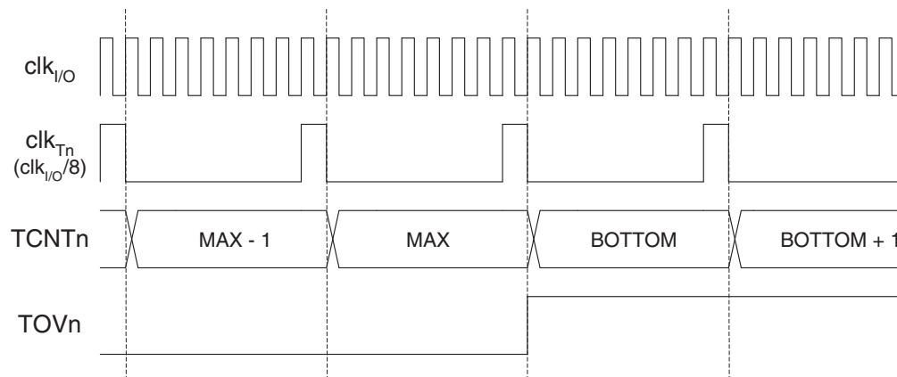
Figure 14-4. Timer/Counter Timing Diagram, with Prescaler ( f_{\text{clk}_{I/O}}/8 )
