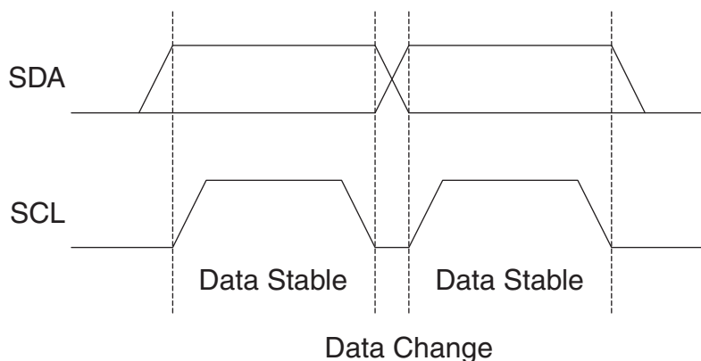
Figure 20-3. Data Validity
