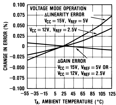
Gain and Linearity Error Variation vs. Temperature
