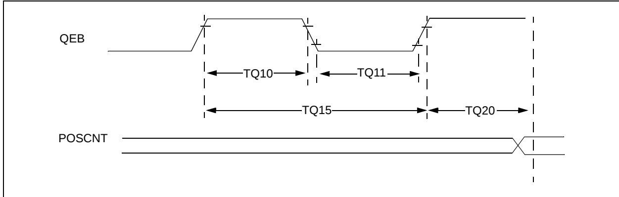
FIGURE 23-8: TIMERQ (QE1 MODULE) EXTERNAL CLOCK TIMING CHARACTERISTICS
