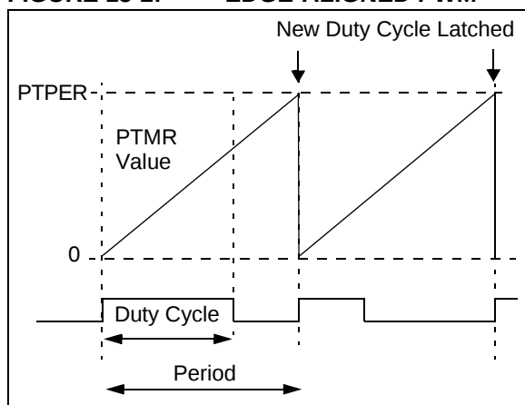
FIGURE 15-2: EDGE-ALIGNED PWM
