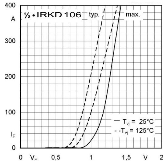
Fig. 15 Forward characteristics
