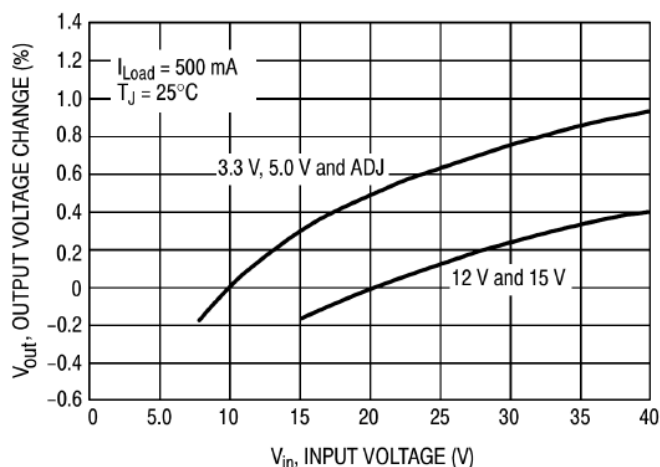
Figure 3. Line Regulation
