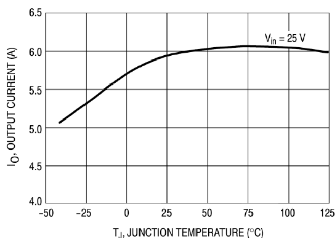
Figure 5. Current Limit
