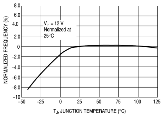
Figure 10. Oscillator Frequency
