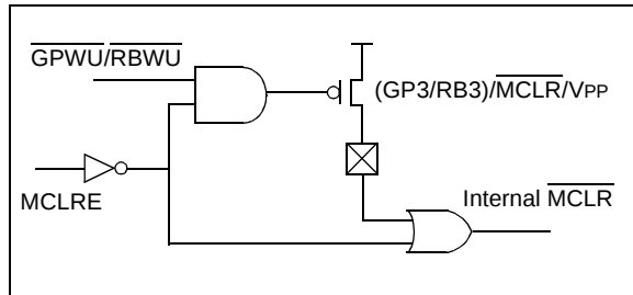
FIGURE 7-7: MCLR SELECT
