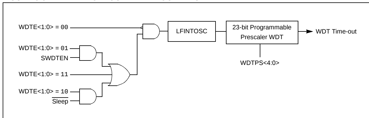
FIGURE 3-3: WATCHDOG TIMER BLOCK DIAGRAM
