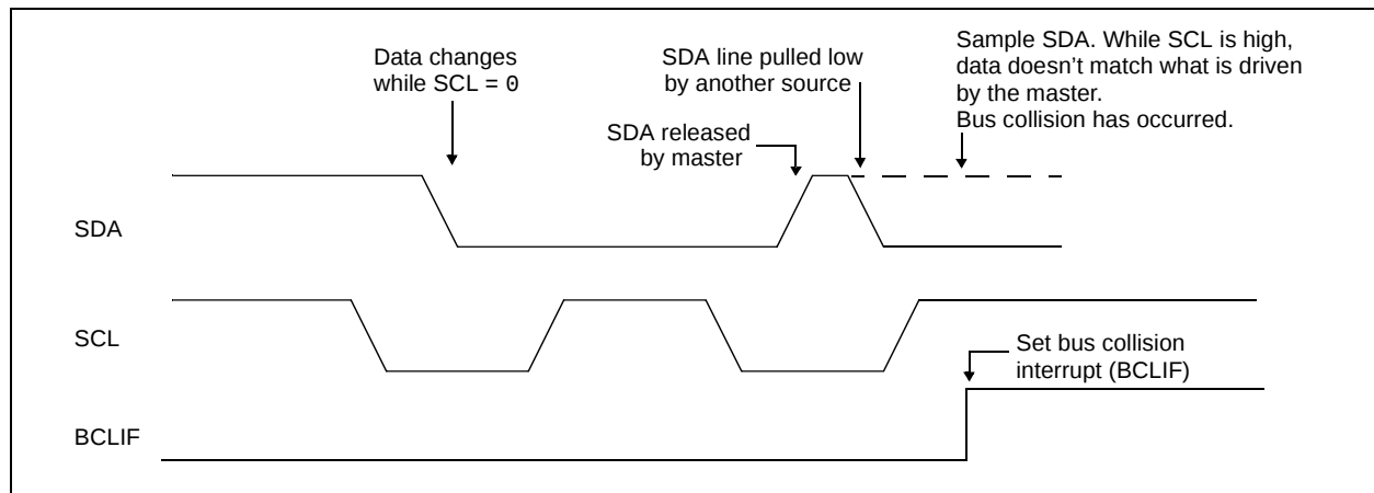
FIGURE 22-29: BUS COLLISION TIMING FOR TRANSMIT AND ACKNOWLEDGE
