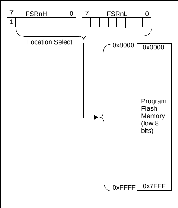
FIGURE 2-8: PROGRAM FLASH MEMORY MAP
