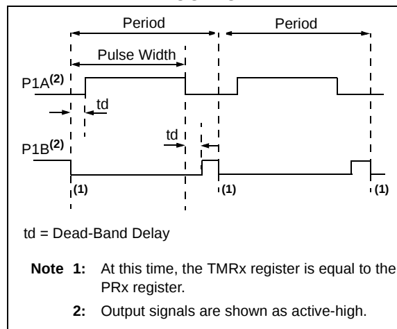
FIGURE 19-16: EXAMPLE OF HALF-BRIDGE PWM OUTPUT
