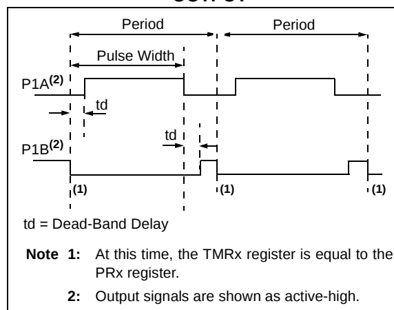
FIGURE 19-8: EXAMPLE OF HALF-BRIDGE PWM OUTPUT
