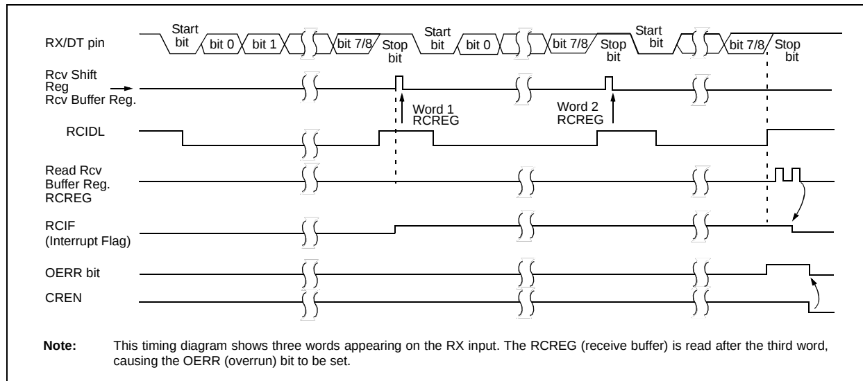
FIGURE 20-5: ASYNCHRONOUS RECEPTION
