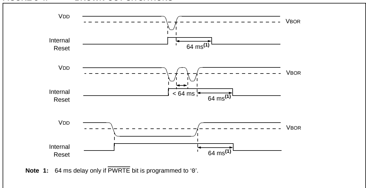
FIGURE 3-4: BROWN-OUT SITUATIONS
