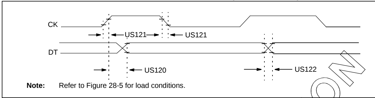
FIGURE 28-14: USART SYNCHRONOUS TRANSMISSION (MASTER/SLAVE) TIMING
