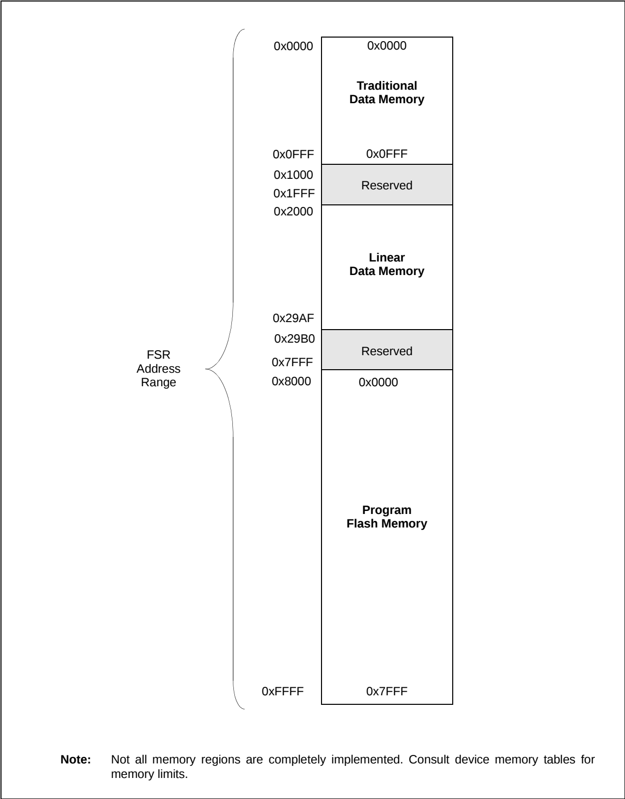
FIGURE 2-5: INDIRECT ADDRESSING
