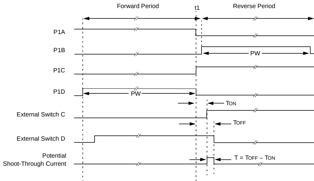
FIGURE 19-13: EXAMPLE OF PWM DIRECTION CHANGE AT NEAR 100% DUTY CYCLE
