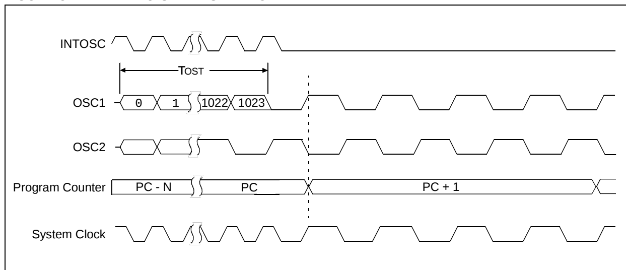
FIGURE 8-7: TWO-SPEED START-UP
