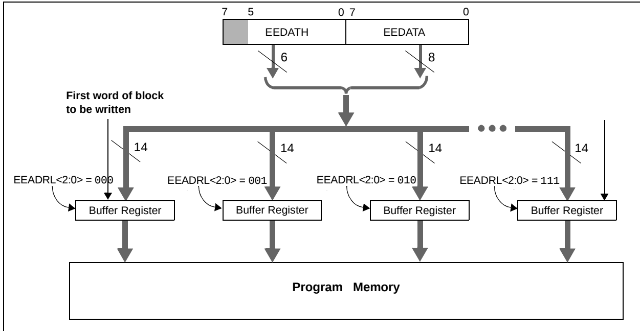
FIGURE 23-2: BLOCK WRITES TO 8K FLASH PROGRAM MEMORY
