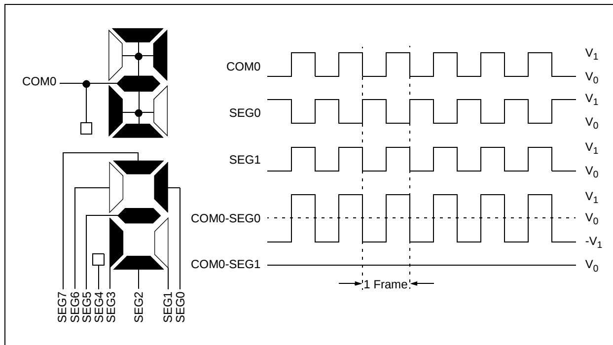
FIGURE 21-7: TYPE-A/TYPER-B WAVEFORMS IN STATIC DRIVE
