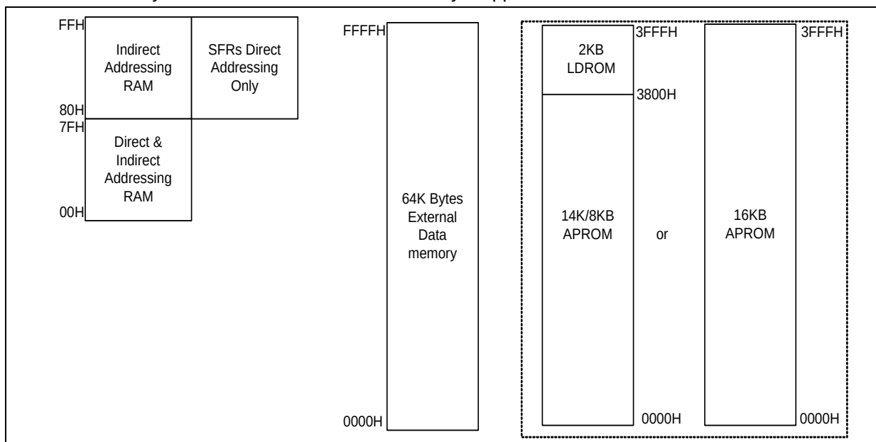
Figure 8-1 Memory Map
