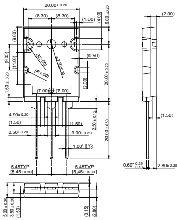
Fig.76 (TO-264)
