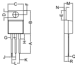
Fig.77 (TO-220AB)
