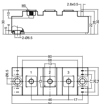
Fig. 1 (C1)
