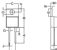
Fig.78 (TO-220AC)
