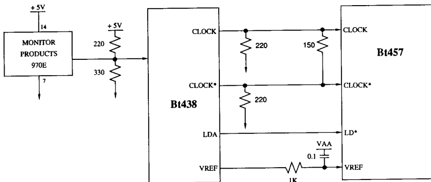
Figure 6. Generating the Bt457 Clock Signals (Monochrome Application).
