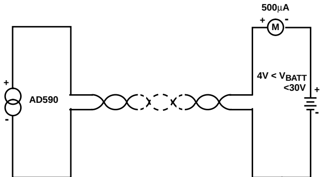
FIGURE 10. SIMPLEST THERMOMETER
