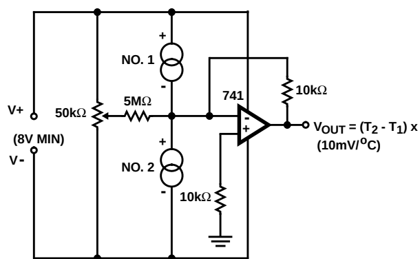
FIGURE 15. DIFFERENTIAL THERMOMETER
