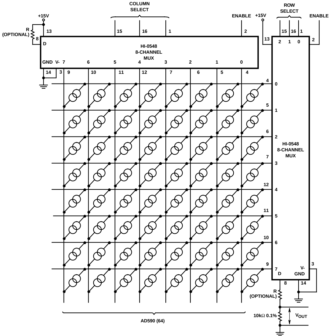
FIGURE 17. MULTIPLEXING SENSORS
