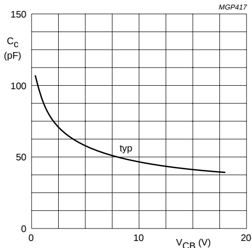
Fig.5 I_E = I_e = 0 ; f = 1\text{ MHz} ; T_j = 25^\circ\text{C} .
