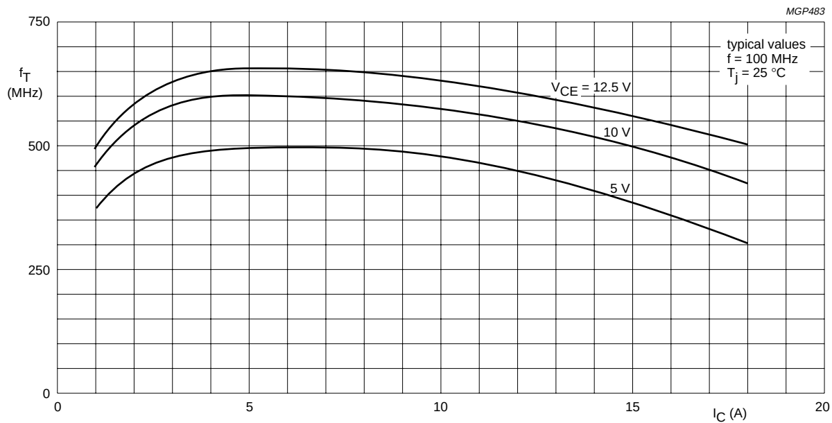
Fig. 6 Transition frequency as a function of collector current.
