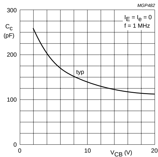
Fig. 5 Collector capacitance as a function of collector-base voltage.
