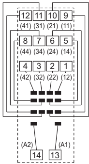
Terminal Arrangement/Internal Connection Diagram
