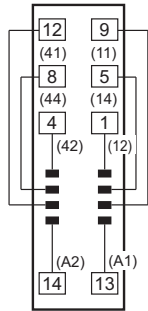
Terminal Arrangement/Internal Connection Diagram
