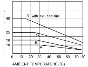
Derating Curve
