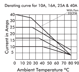
Derating Curve
