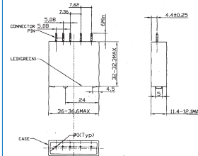
Mechanical Drawing
