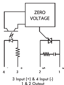
Schematic
