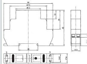
Mechanical Drawing
