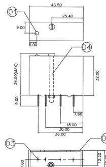
Mechanical Drawing
