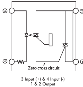
Schematic
