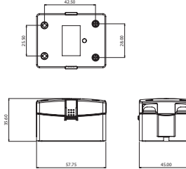
Mechanical Drawing
