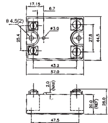
Mechanical Drawing
