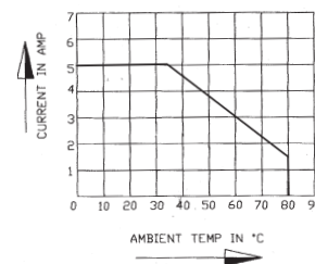
Derating Curve
