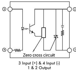
Schematic
