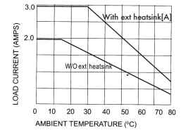
Derating Curve
