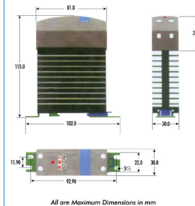
Mechanical Drawing
