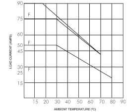
Derating Curve
