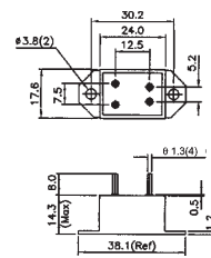
Mechanical Drawing
