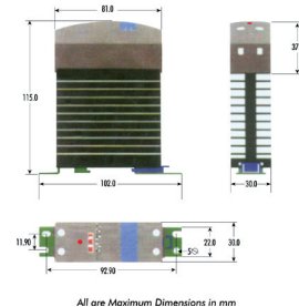
Mechanical Drawing
