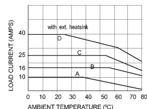
Derating Curve
