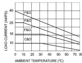
Derating Curve
