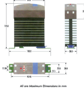
Mechanical Drawing
