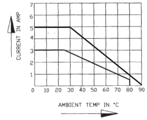
Derating Curve
