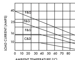
Derating Curve
