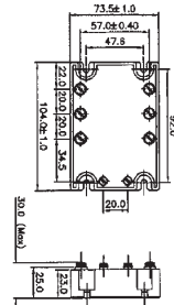
Mechanical Drawing
