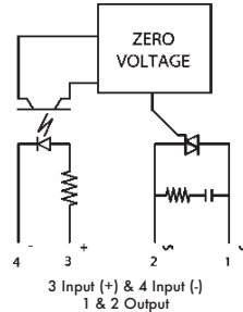
Schematic
