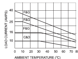
Derating Curve
