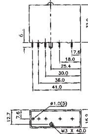
Mechanical Drawing
