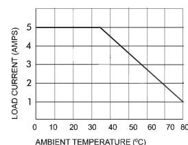
Derating Curve
