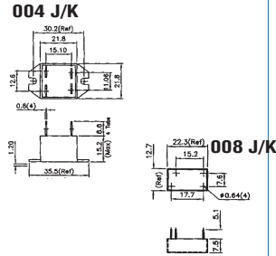
Mechanical Drawing
