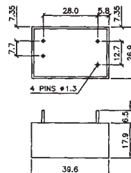
Mechanical Drawing
