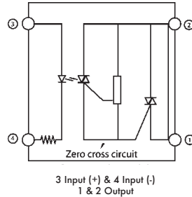
Schematic
