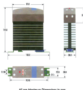
Mechanical Drawing
