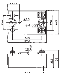
Mechanical Drawing
