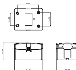
Mechanical Drawing
