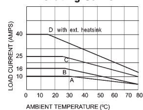
Derating Curve
