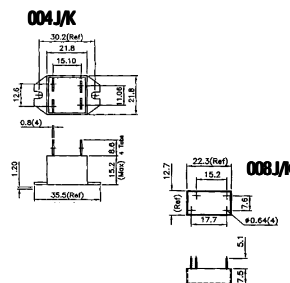
Mechanical Drawing
