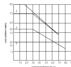
Derating Curve
