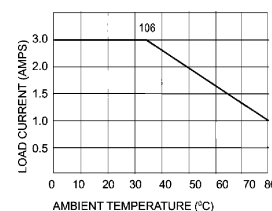
Derating Curve
