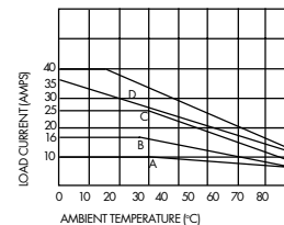
Derating Curve
