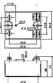
Mechanical Drawing
