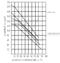
Derating Curve
