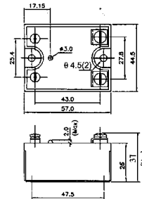
Mechanical Drawing
