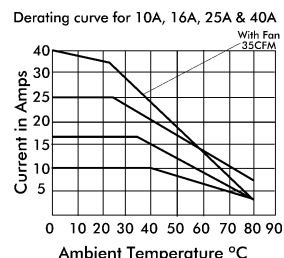
Derating Curve
