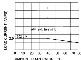
Derating Curve
