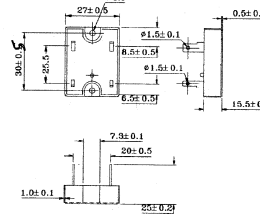
Mechanical Drawing
