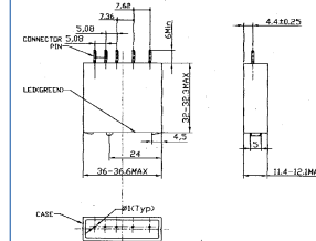
Mechanical Drawing
