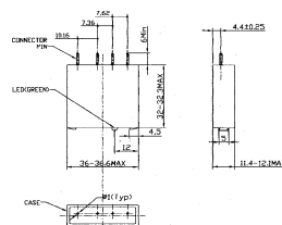
Mechanical Drawing
