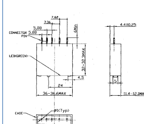
Mechanical Drawing
