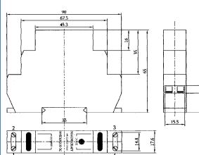
Mechanical Drawing
