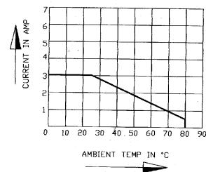
Derating Curve
