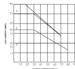
Derating Curve
